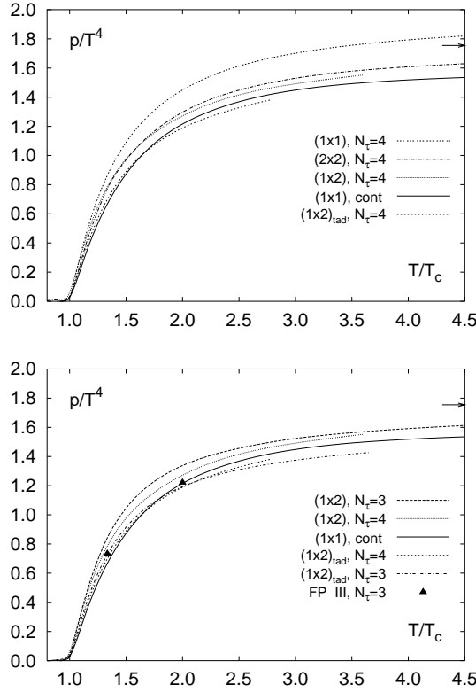
Fig. 4. Pressure of the SU(3) gauge theory calculated with the Wilson action and different improved actions on N_\tau = 4 lattices (upper figure). The lower figure shows a comparison of calculations with tree level and tadpole improved actions on N_\tau = 3 and 4 lattices. Also shown there are results from a calculation with a fixed point action (triangles). The arrows indicate the ideal gas result in the continuum limit. For comparison we also show the continuum extrapolation obtained from calculations with the Wilson action [3]
