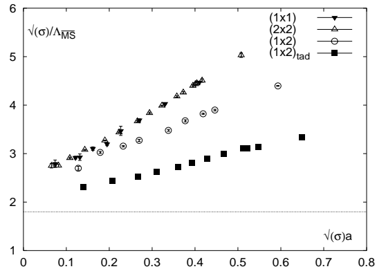
Fig. 2. \sqrt{\sigma}/\Lambda_{\overline{\text{MS}}} versus \sqrt{\sigma}a for various actions. Shown are results for \sqrt{\sigma}a/R(g^2) , normalized to \Lambda_{\overline{\text{MS}}} . Here R(g^2) denotes the 2-loop \beta -function. In the case of the (2,2)-action the ratio of \Lambda_{\text{tree}}^{(2,2)}/\Lambda_{\overline{\text{MS}}} was not known to us and we have, therefore, used an arbitrary normalization factor of 0.15. The horizontal line indicates the value of the continuum extrapolation of \sqrt{\sigma}/\Lambda_{\overline{\text{MS}}} for the Wilson action taken from [6]
