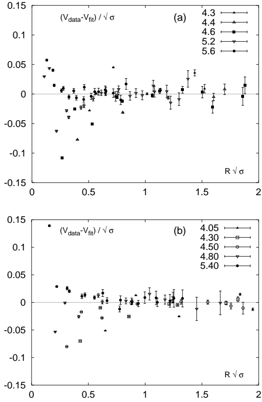
Fig. 1. The difference between the calculated potentials and the best fit obtained with fixed \hat{\alpha} in units of \sqrt{\hat{\sigma}} versus R\sqrt{\hat{\sigma}} . Shown are results for the tree level improved (2,2)-action (a) and the tadpole improved (1,2)-action (b) for different values of the gauge coupling. Tree level results for the latter action look similar
