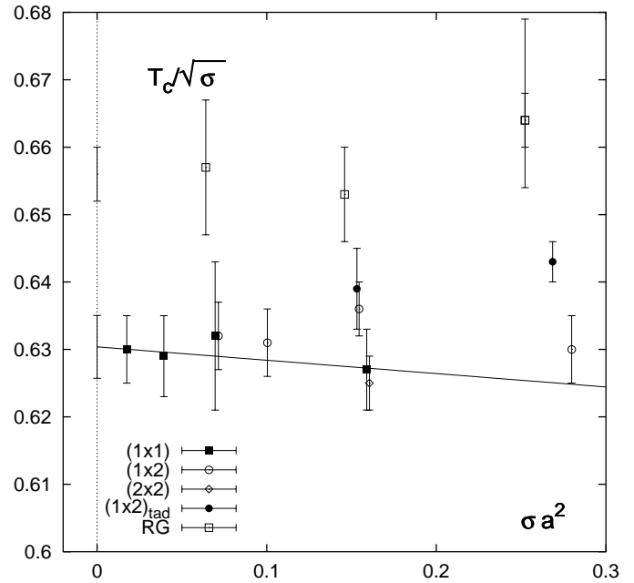
Fig. 3. The critical temperature in units of the square root of the string tension for various actions versus the square of the cut-off. The N_\tau = 6 point of the tree level (1,2) improved action has been slightly shifted to make it distinguishable from the Wilson action point
