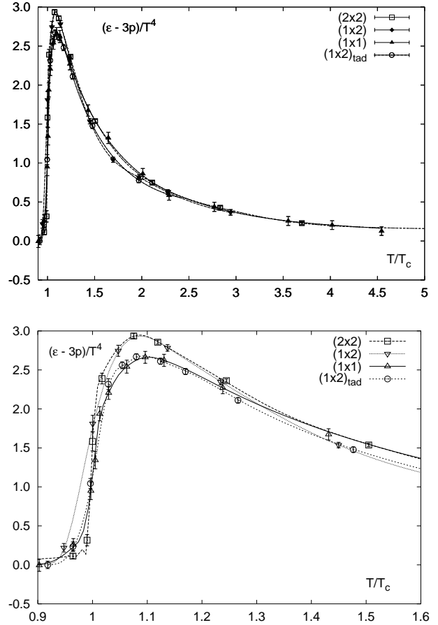
Fig. 5. The difference (\epsilon - 3p)/T^4 versus T/T_c calculated on lattices with temporal extent N_\tau = 4 for various improved actions. The results are compared to a calculation with the Wilson action on a N_\tau = 8 lattice. In the lower figure the peak of (\epsilon - 3p)/T^4 is shown in detail
